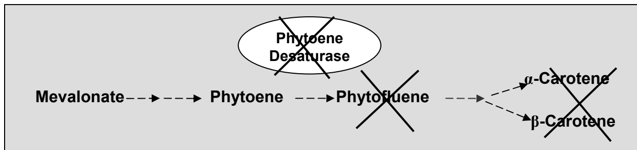
Figure 1. Fluridone mode of action in the carotenoid biosynthetic pathway of newly emerging tissue
